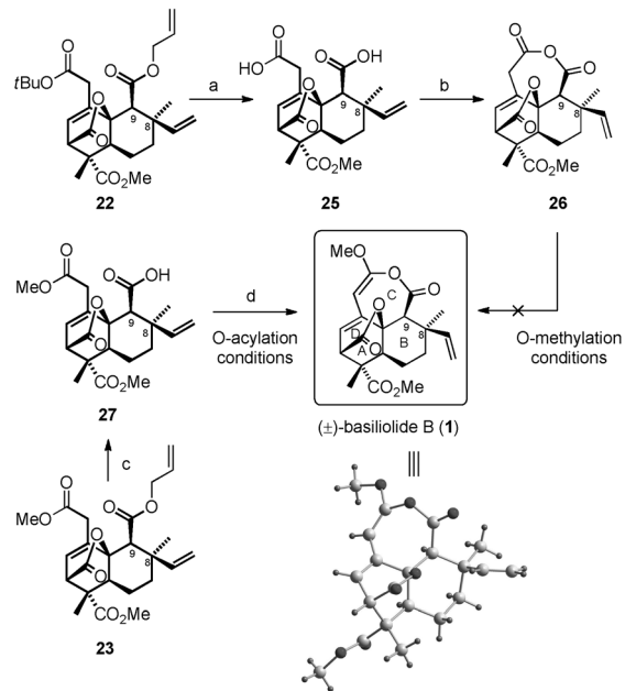
Scheme 3. Biomimetic approaches toward the C ring formation and total synthesis of (±)-basiliolide B. a) Pd(PPh 3 ) 4 , PPh 3 , pyrrolidine, CH 2 Cl 2 , 0°C, 2.5 h; then HCO 2 H, RT, 10 h (90%); b) EDCl, DMAP, CH 2 Cl 2 , RT, 4 h (70%); c) Pd(PPh 3 ) 4 , PPh 3 , pyrrolidine, CH 2 Cl 2 , 0°C, 30 min (96%); d) Tf 2 O, Et 3 N, toluene, –78 for 10 min and 0°C for 5 min (92%). EDCl = 1-ethyl-3-(3-dimethylaminopropyl)carbodiimide hydrochloride, DMAP = N,N -4-dimethylaminopyridine.
